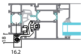
Vindushengsle, synlig WICSTAR aluminium
