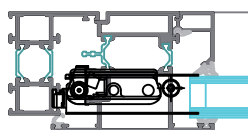
Vindushengsle, skjult WICSTAR aluminium
